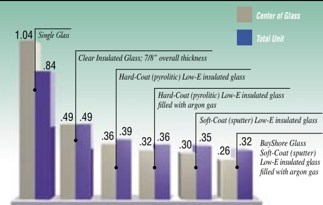
U-Factor Comparison
